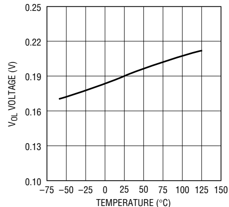
V_{OL} ( \overline{\text{RESET}}n , \overline{\text{FAULT}} ) vs Temperature
