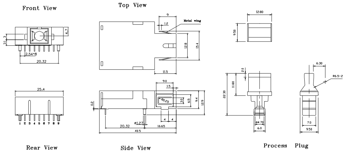
BTR-7710G / BTR-7710AG
