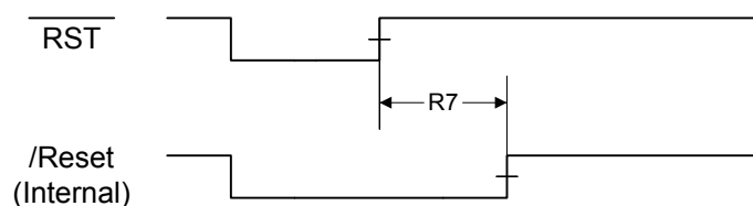
Figure 16-5. External Reset Timing (RST)
