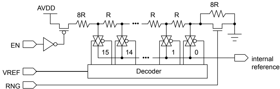
Figure 12-3. Comparator Internal Reference Structure
