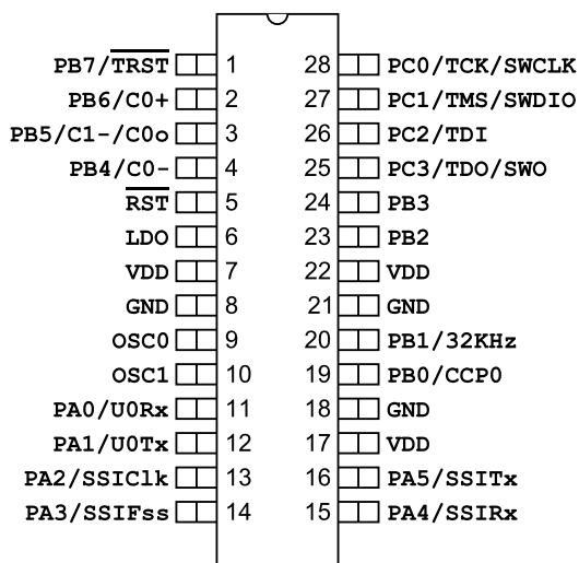
LM3S101
