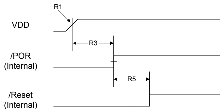
Figure 16-6. Power-On Reset Timing
