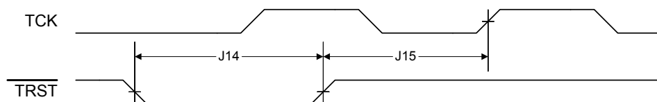
Figure 16-4. JTAG TRST Timing
