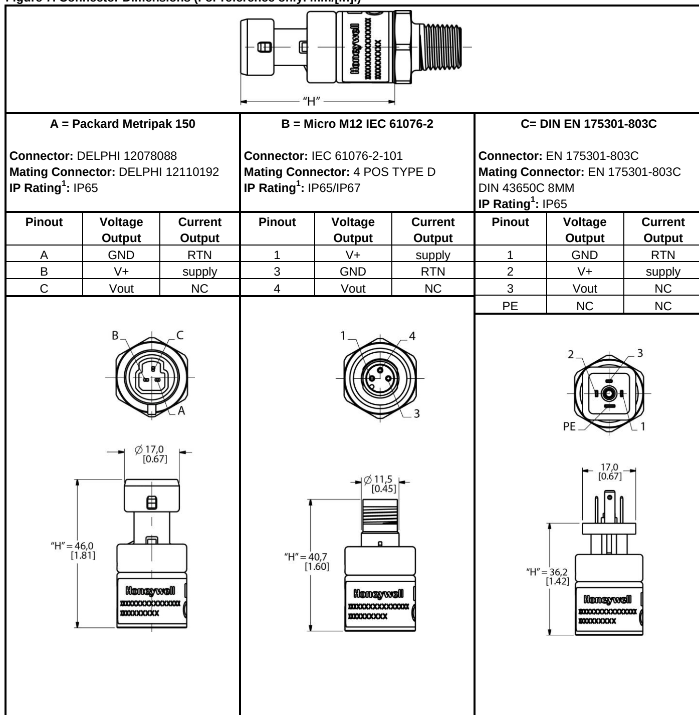
Figure 7. Connector Dimensions (For reference only: mm/[in].)
