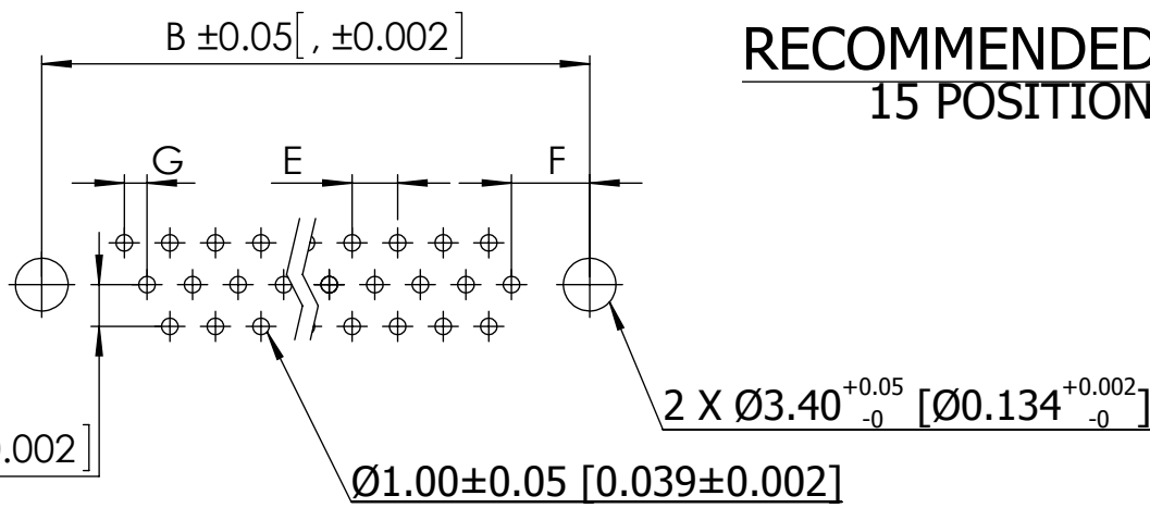
RECOMMENDED PCB LAYOUT 26,44,62 POSITIONS FEMALE
