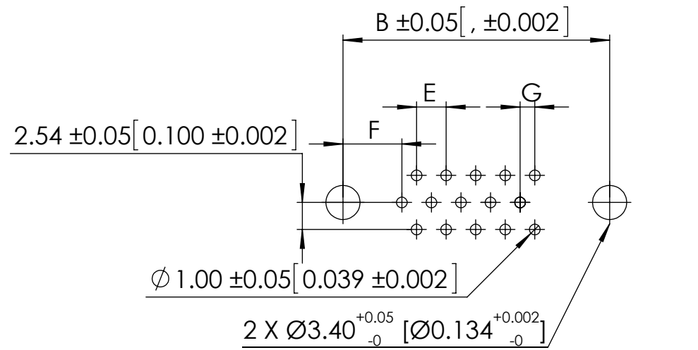
RECOMMENDED PCB LAYOUT 15 POSITIONS MALE
