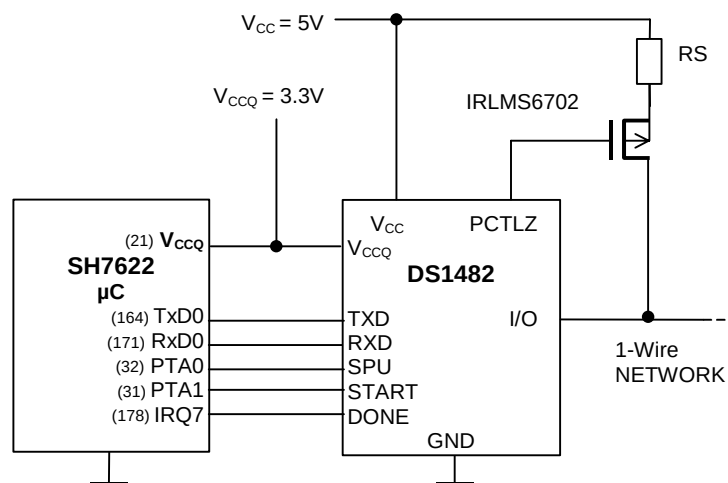
Figure 2. Typical Operating Circuit
