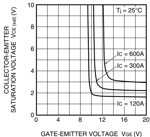
COLLECTOR-EMITTER SATURATION VOLTAGE CHARACTERISTICS
