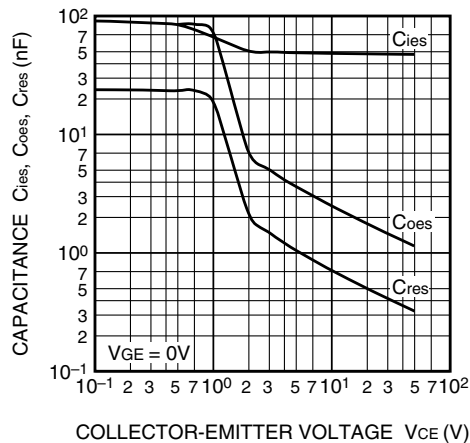
CAPACITANCE-VCE CHARACTERISTICS
