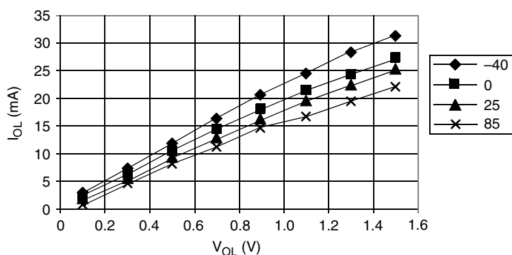
Figure 23-10. Typical Low-Side Driver Characteristics – Port PTC1-PTC0 ( V_{DD} = 2.7 Vdc)
