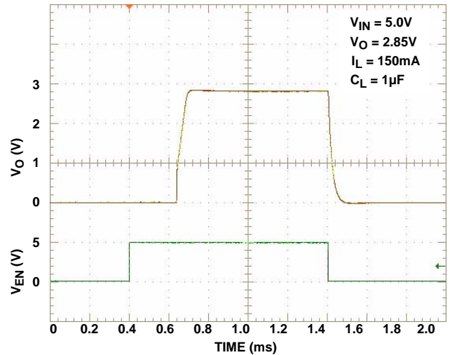
FIGURE 12. TURN-ON/TURN-OFF RESPONSE
