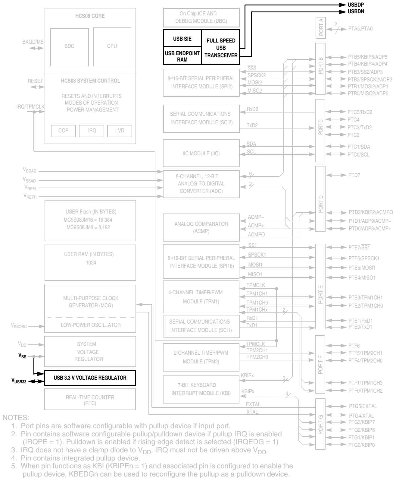
Figure 17-1. MC9S08JM16 Series Block Diagram Highlighting USB Blocks and Pins
