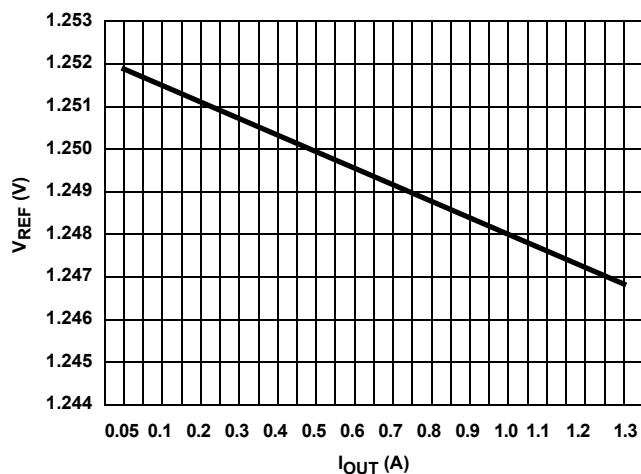
FIGURE 12. V REF vs OUTPUT CURRENT at T A = +25 °C
