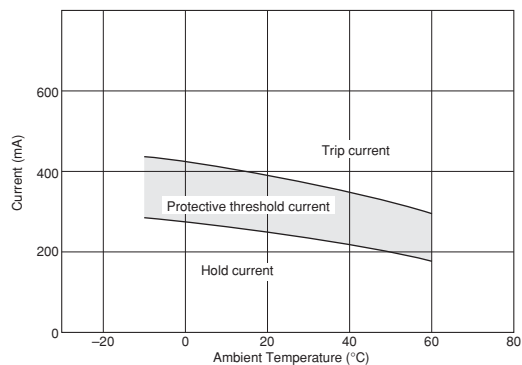
PTGL14AR180M9C01B0
