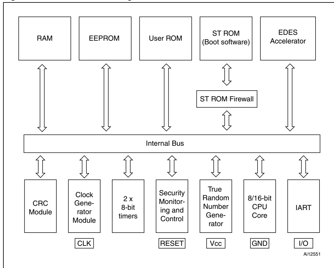
Figure 1. ST23YS02 block diagram
