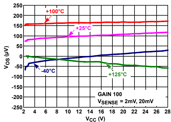
FIGURE 10. V_{OS} vs V_{CC} , V_{RS+} = 12V
