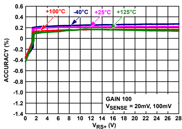
FIGURE 12. GAIN ACCURACY vs V_{RS+} = 0V TO 28V
