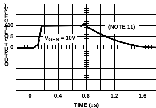
FIGURE 2C. V_{ANALOG} = 10V
