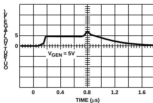
FIGURE 2D. V_{ANALOG} = 5V
