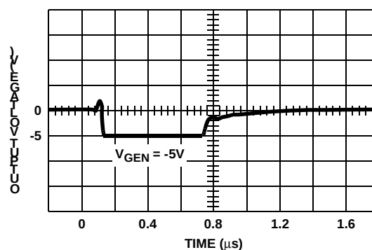
FIGURE 2F. V_{ANALOG} = -5V
