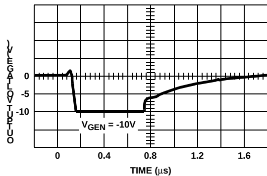
FIGURE 2G. V_{ANALOG} = -10V
