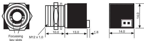
Figure 1 Mechanical details
