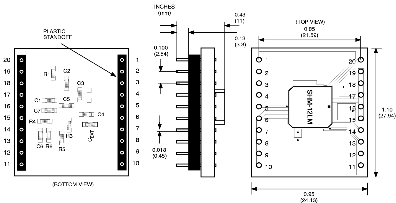
Figure 5. SHM-14 Evaluation Board Dimensions
