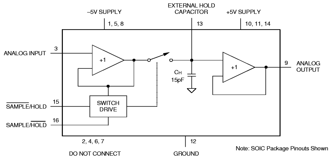
Figure 1. SHM-14 Functional Block Diagram
