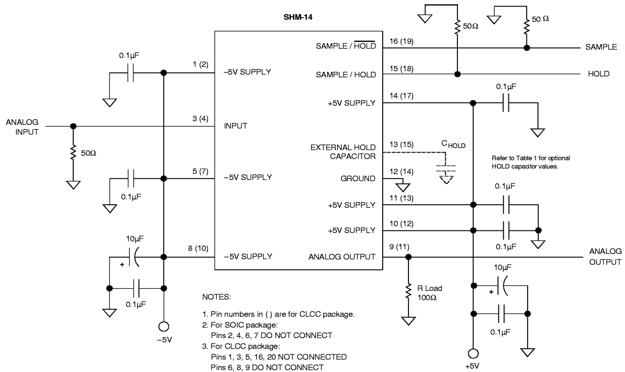
Figure 2. SHM-14 Simplified Connection Diagram
