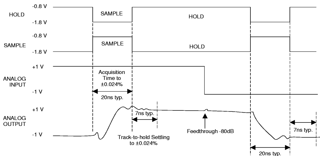
Figure 3. SHM-14 Control and Timing
