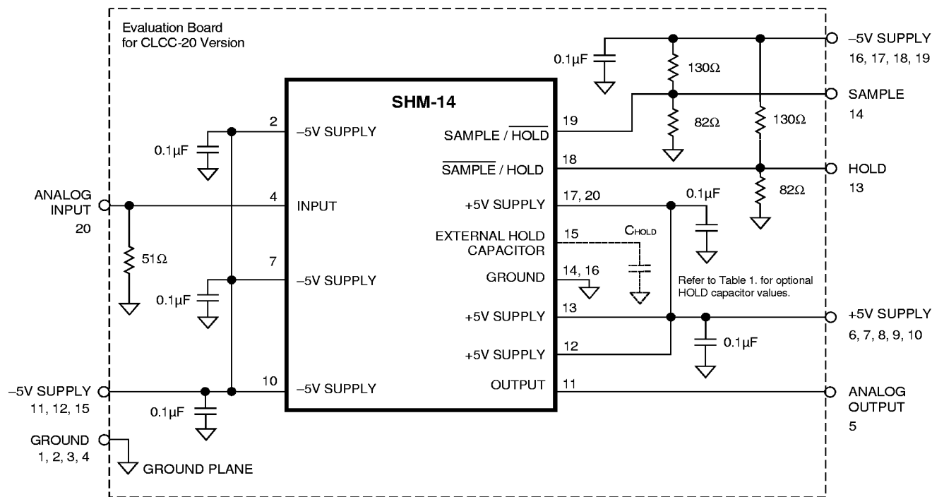
Figure 4. SHM-14 Evaluation Board Schematic
