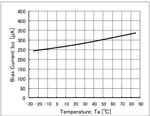
Figure 7. T_a - I_{cc}
