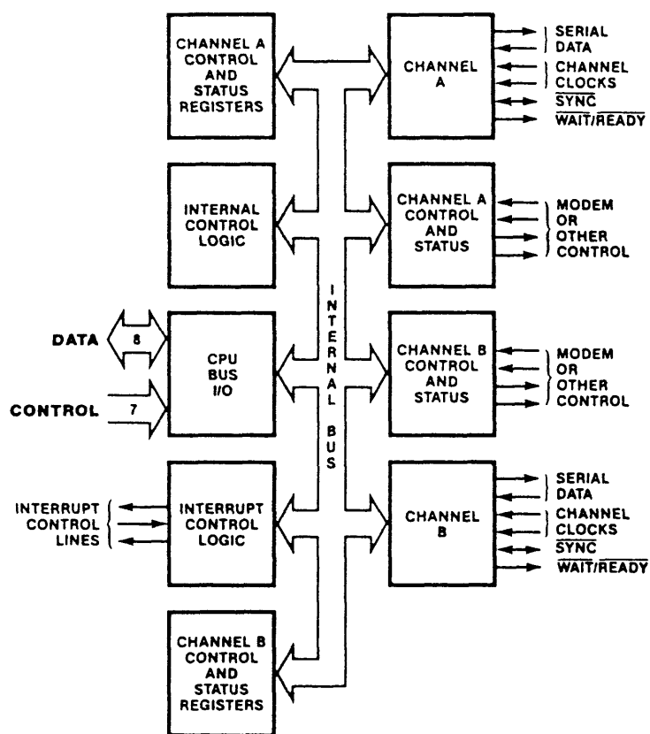
Figure 8. Block Diagram
