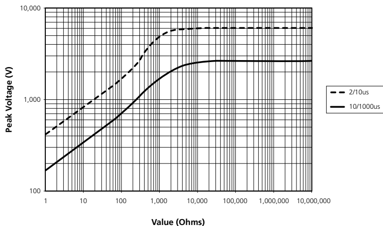
DSC2512 - Bellcore GR1089 Lightning Surge
