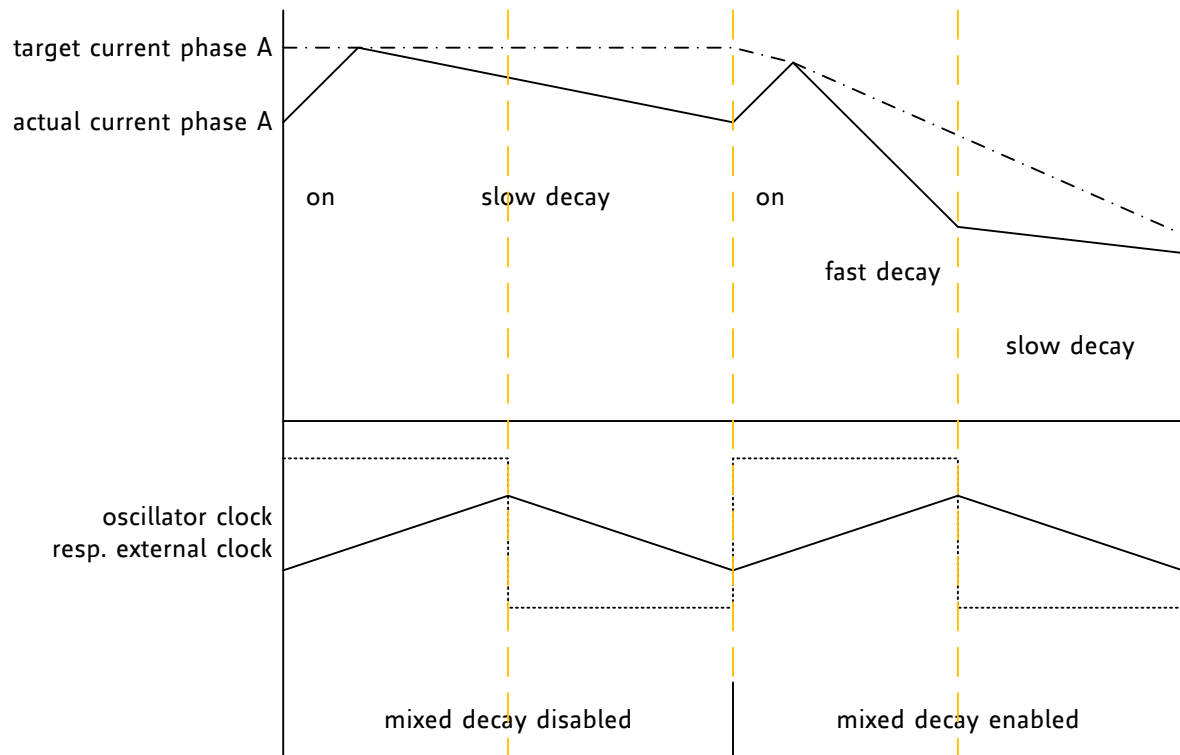
Figure 7.2 Chopper cycle
