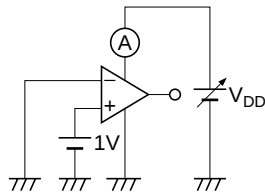
1. Supply Current, I_{DD} (Output High)
