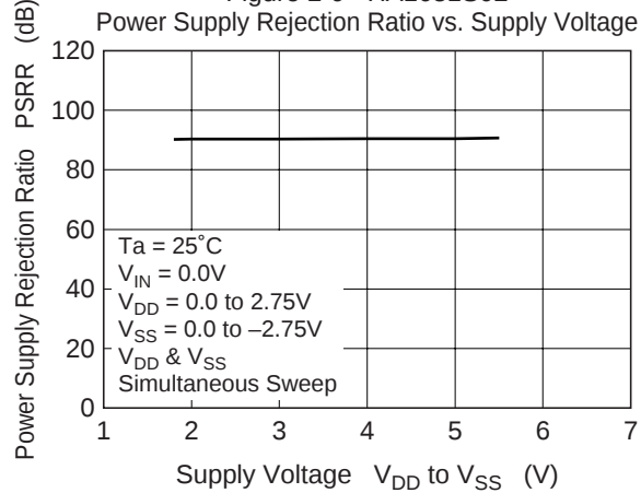
Figure 2-9 HA1631S02
