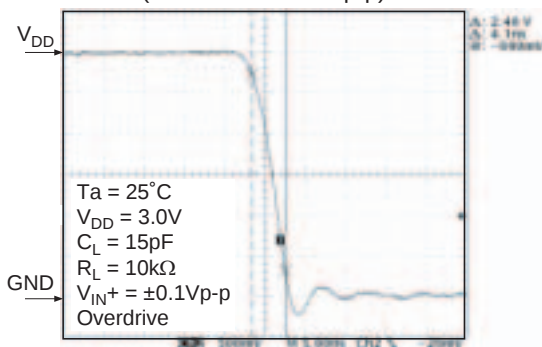
Figure 4-15 HA1631S04 Falling Time, t_f (Overdrive = \pm 0.1\text{Vp-p} )
