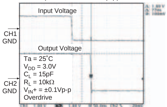
Figure 4-17 HA1631S04 TP_{HL} Transient Response (Overdrive = \pm 0.1\text{Vp-p} )
