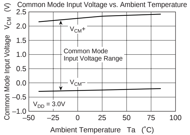
Figure 2-8 HA1631S02
