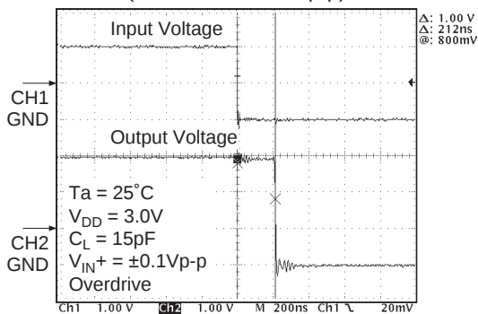
Figure 3-17 HA1631S03 TP_{HL} Transient Response (Overdrive = \pm 0.1\text{Vp-p} )
