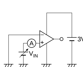
10. Input Bias Current, I_{IB}
