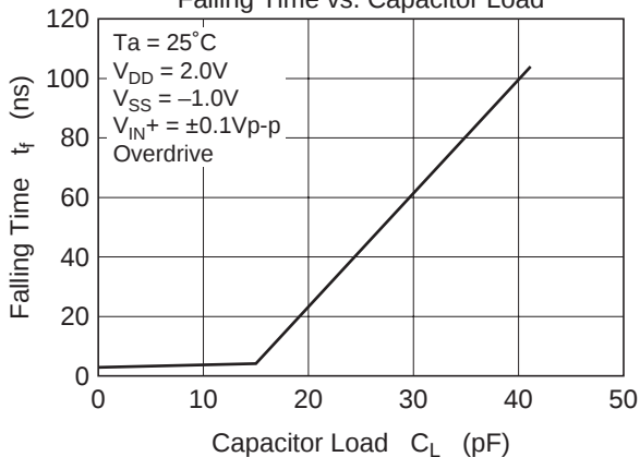
Figure 4-15 HA1631S04 Falling Time, t_f (Overdrive = \pm 0.1\text{Vp-p} )
