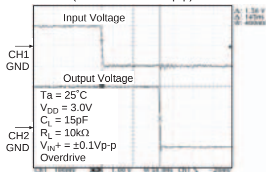
Figure 4-16 HA1631S04 TP_{HL} Transient Response (Overdrive = \pm 0.1\text{Vp-p} )
