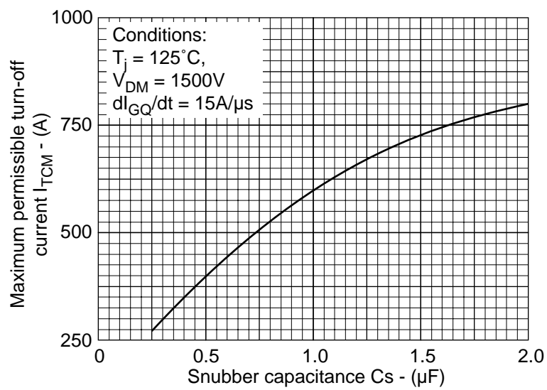
Fig.3 Dependence of I_{TCM} on C_s
