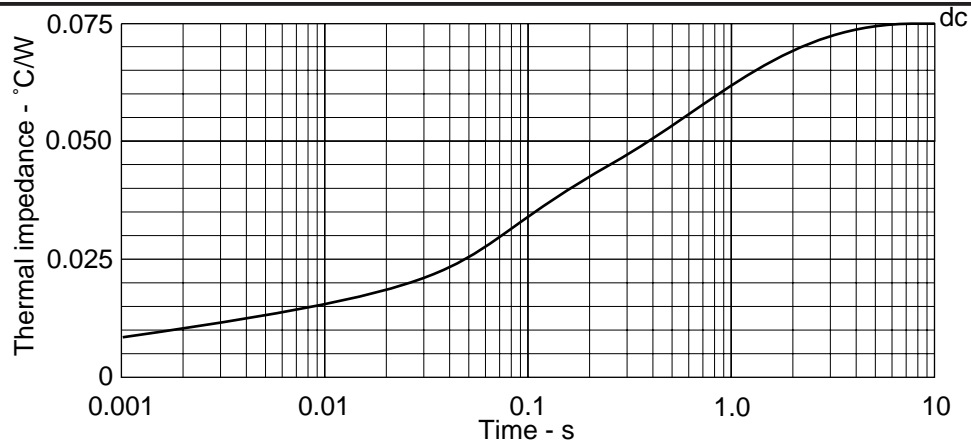
Fig.4 Maximum (limit) transient thermal impedance - double side cooled
