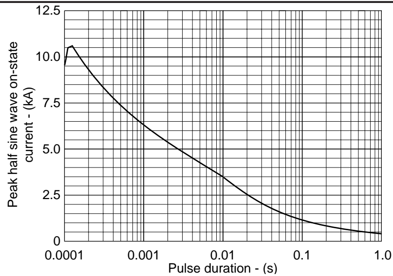
Fig.5 Surge (non-repetitive) on-state current vs time
