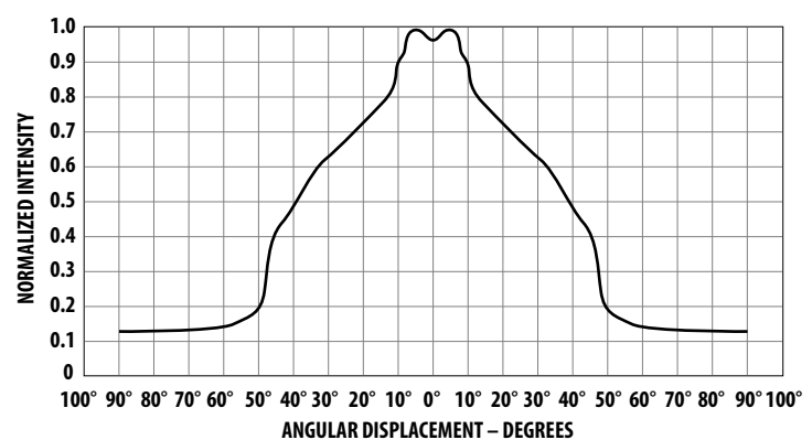
Figure 10: HLMP-P106/-P156
