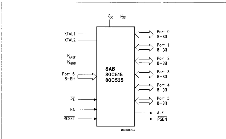
Logic Symbol
