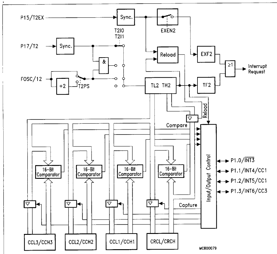
Figure 3 Block Diagram of Timer/Counter 2
