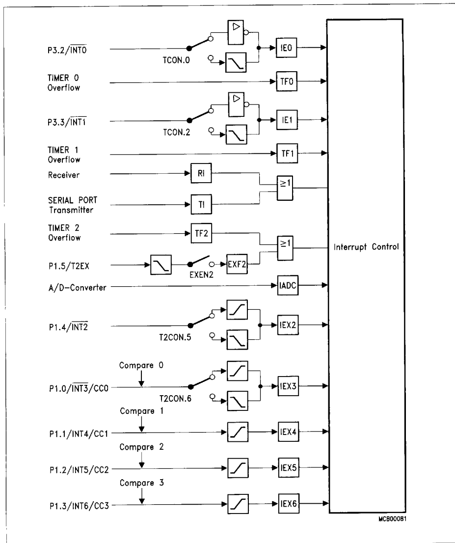
Figure 5 Interrupt Request Sources
