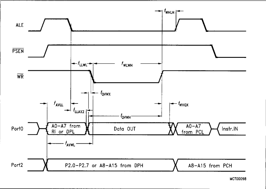
Data Memory Write Cycle
