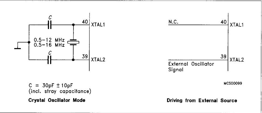
Recommended Oscillator Circuits
