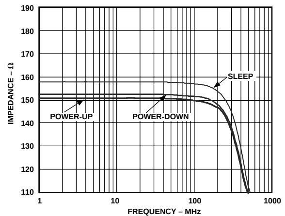
TPC 10. Input Impedance vs. Frequency (Inputs Shunted with 165 Ω)
