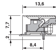
Dimensional drawing
