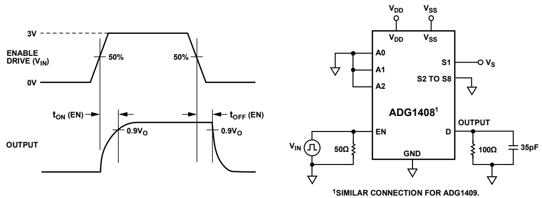
Figure 31. Enable Delay, t_{\text{ON}}(\text{EN}) , t_{\text{OFF}}(\text{EN})
