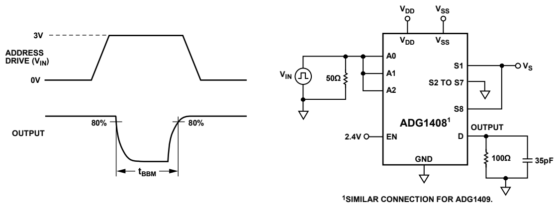
Figure 30. Break-Before-Make Delay, t_{\text{BBM}}
