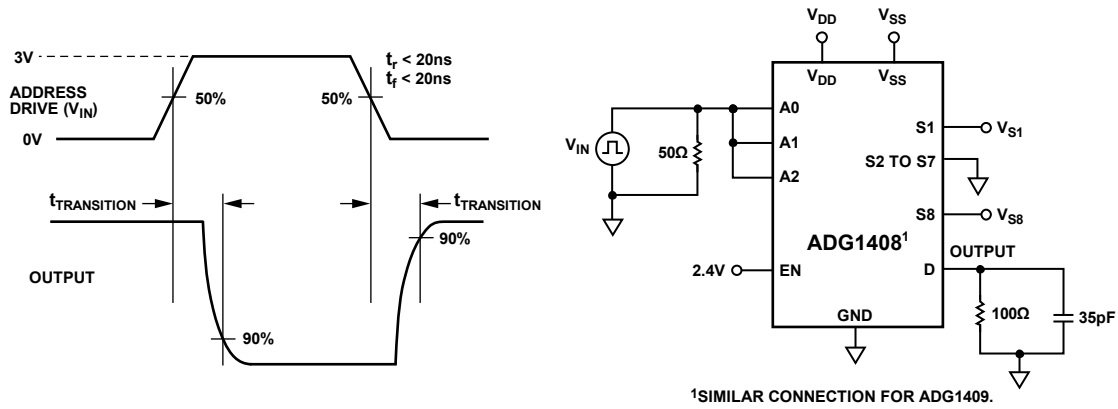
Figure 29. Address to Output Switching Times, t_{\text{TRANSITION}}
