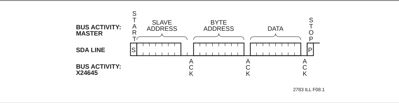
Figure 5. Byte Write
