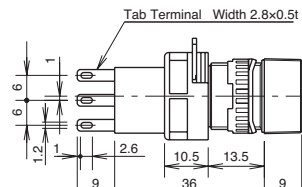
Solder/Tab Terminal
