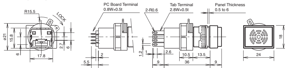
Solder/Tab Terminal
