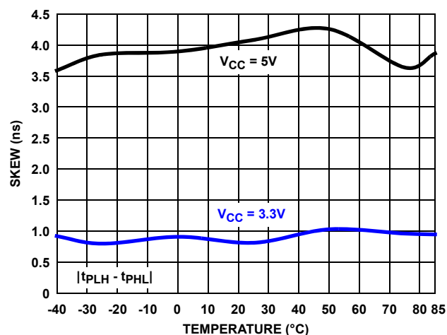
FIGURE 18. DRIVER DIFFERENTIAL SKEW vs TEMPERATURE (ISL32453E, ISL32455E)
