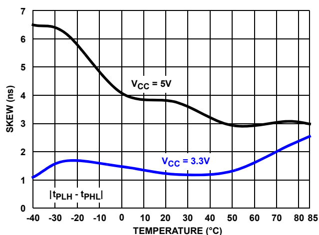
FIGURE 16. DRIVER DIFFERENTIAL SKEW vs TEMPERATURE (ISL32450E, ISL32452E, ISL32457E)
