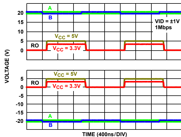
FIGURE 20. \pm 20\text{V} RECEIVER PERFORMANCE (ISL32453E, ISL32455E)
