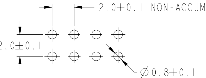
RECOMMENDED HOLE LAYOUT SCALE 5:1
