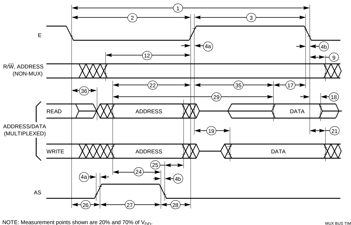
Figure A-8 Multiplexed Expansion Bus Timing Diagram
