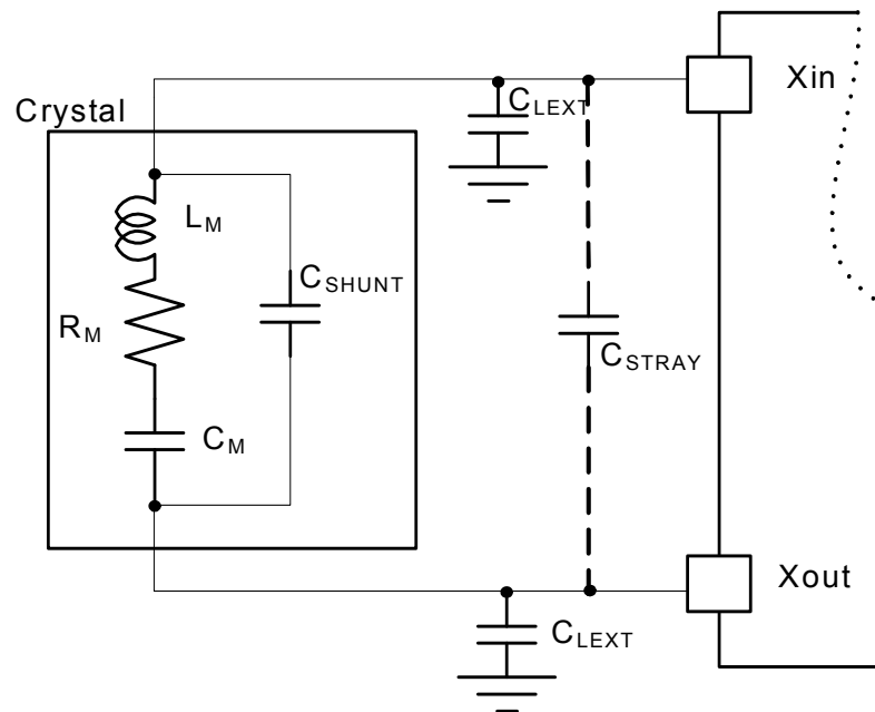
Figure 9-3. Oscillator Connection
