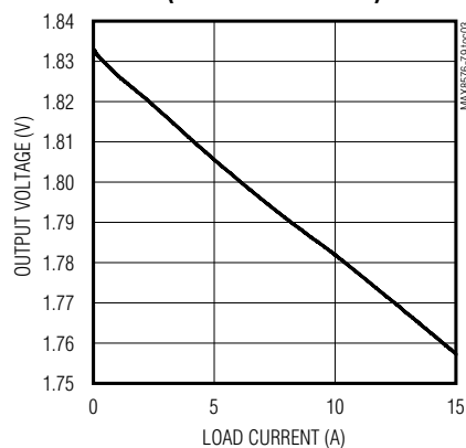
LOAD REGULATION (CIRCUIT OF FIGURE 2)
