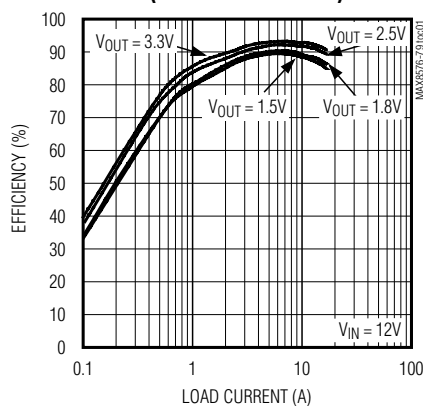
EFFICIENCY vs. LOAD CURRENT (CIRCUIT OF FIGURE 2)
