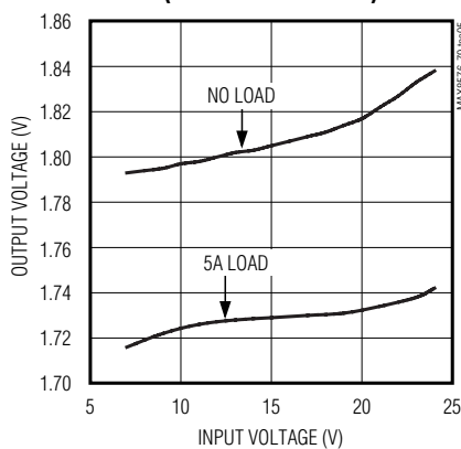
LINE REGULATION (CIRCUIT OF FIGURE 3)
