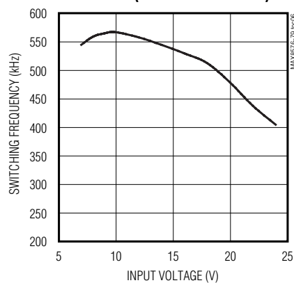
SWITCHING FREQUENCY vs. INPUT VOLTAGE (CIRCUIT OF FIGURE 3)
