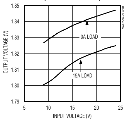
LINE REGULATION (CIRCUIT OF FIGURE 2)
