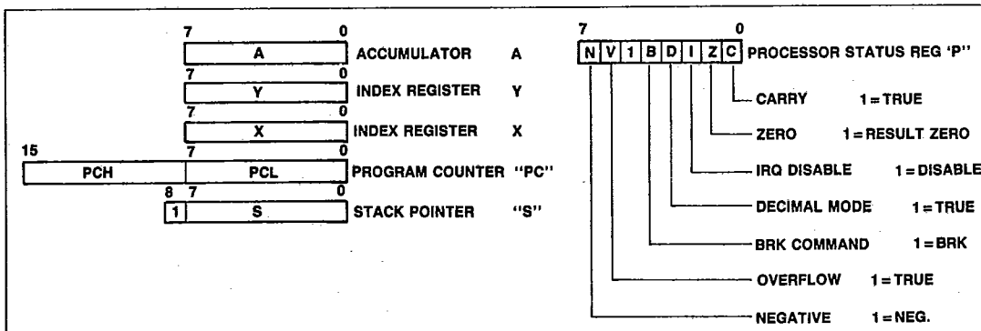
Programming Model
