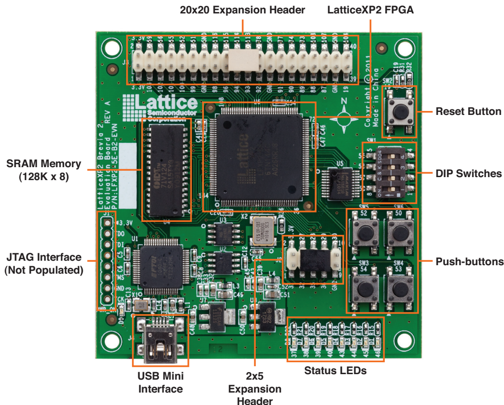
Figure 1. LatticeXP2 Brevia 2 Evaluation Board, Top Side
