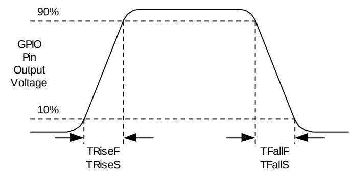
Figure 3-7. GPIO Timing Diagram
