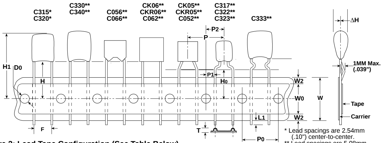
Figure 2: Lead Tape Configuration (See Table Below)
