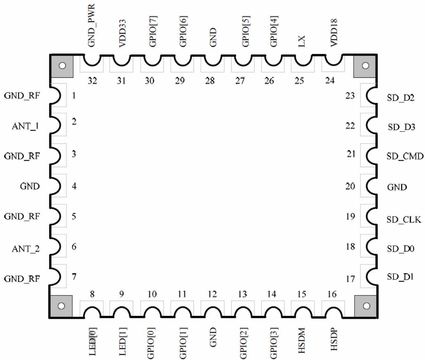
Figure 2: Module Pinout
