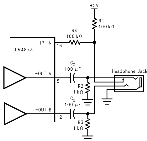
Figure 47. Headphone Circuit
