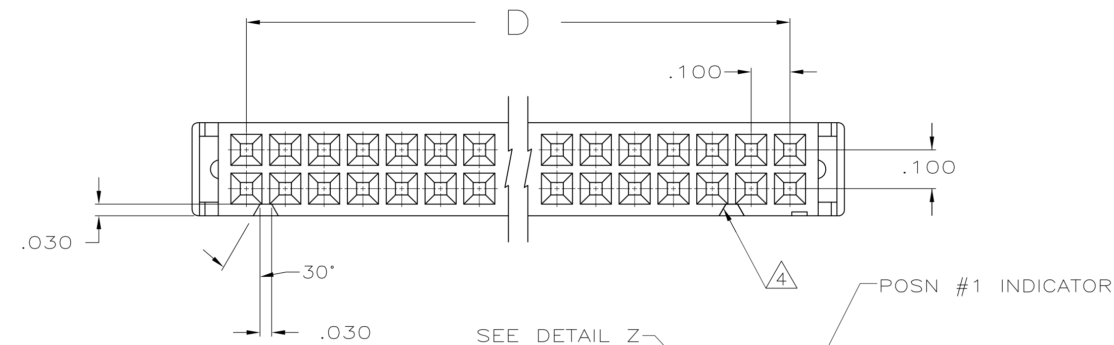
TERMINATED VIEW
