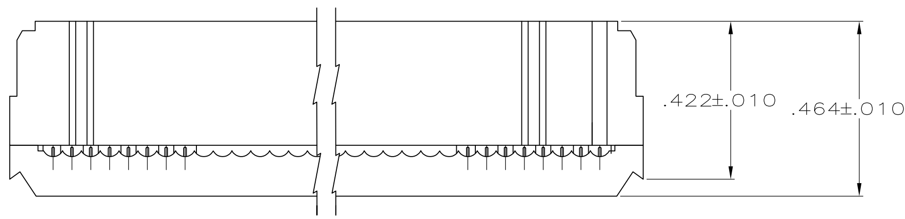
TERMINATED VIEW
