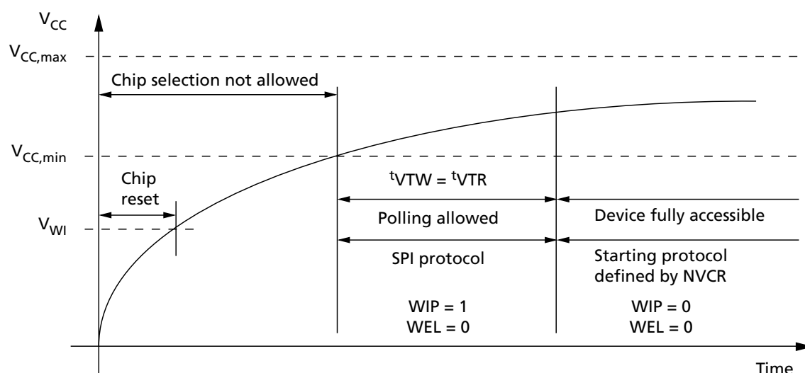
Figure 32: Power-Up Timing
