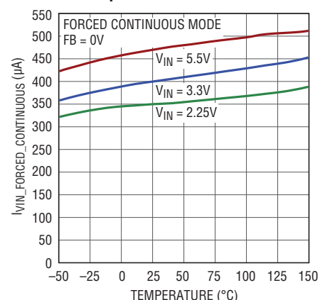
Buck V_{IN} Supply Current vs Temperature
