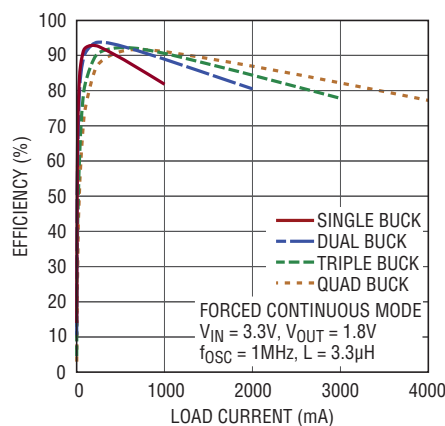
Buck Efficiency vs I L LOAD
