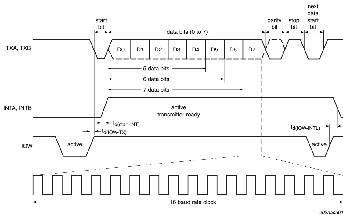
Fig 17. Transmit timing
