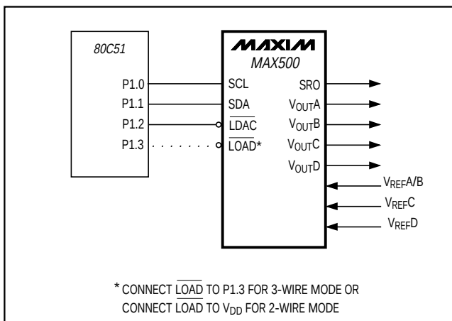
Figure 13. 80C51 Interface
