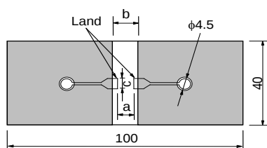
Fig.1 (in mm)
