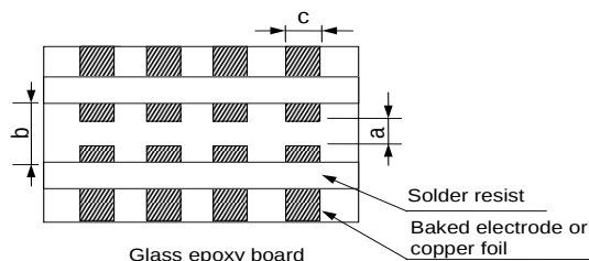
Fig.3 (in mm)
