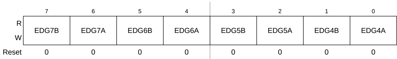
Figure 15-16. Timer Control Register 3 (TCTL3)
