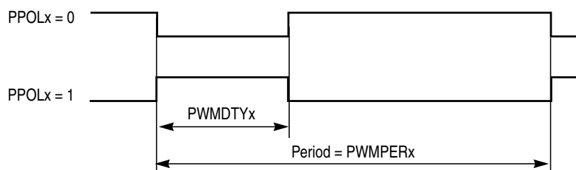
Figure 12-30. PWM Left Aligned Output Waveform
