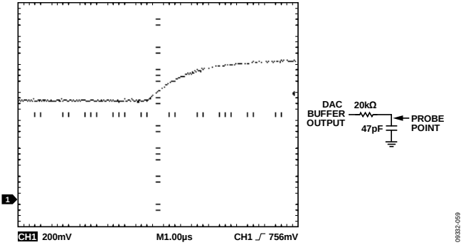
Figure 17. Transient Response of DAC Code Change into Typical Load
