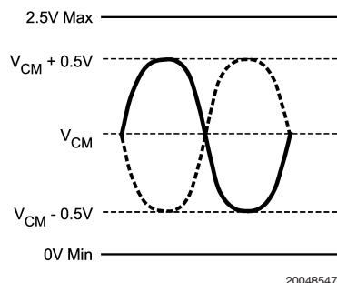
FIGURE 3. Input Voltage Waveforms for a 2V P-P Differential Input
